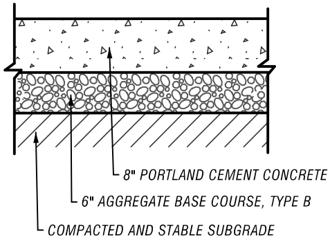
TYPICAL CONCRETE PAVEMENT SECTION LOADING DOCK NOT TO SCALE
